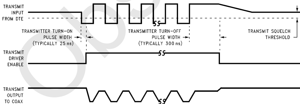
FIGURE 3. Transmitter Timing
