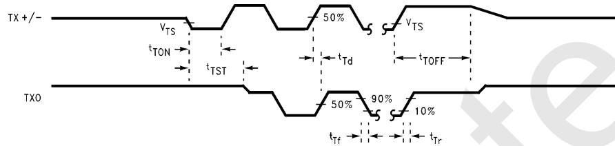
FIGURE 9. Transmitter Timing
